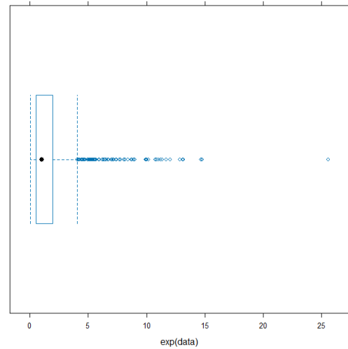
Figure 4: d, Boxplot
