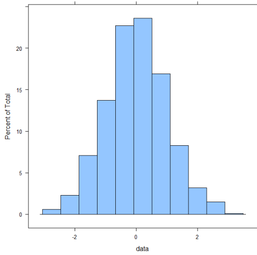
Figure 1: a, Histogram
